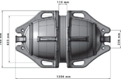
MUSSEL BUOY DIMENSIONS
